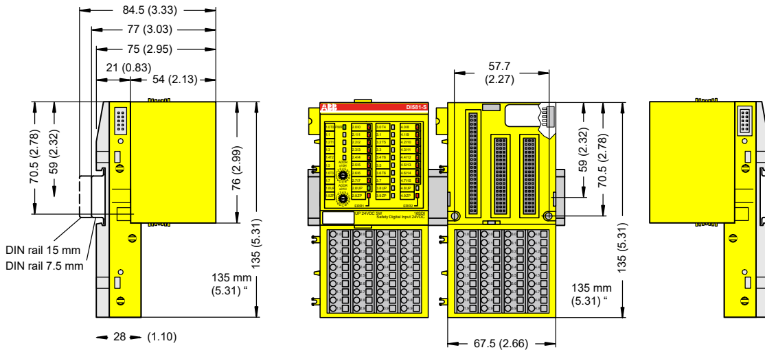
Fig. 1: Dimensions of DI581-S safety I/O module
